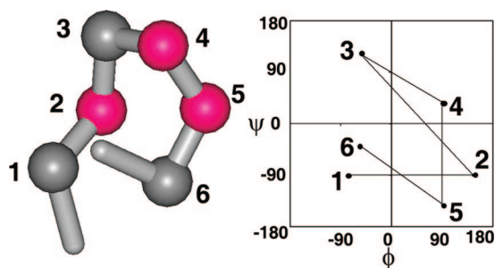
FIGURE 6. A designed peptide aperiodic in stereochemical and conformational structures, showing the fold topology (D residues in red color) and \phi, \psi values in the crystal structure of Boc-LLeu-DVal-LPro-DAsp-DVal-LLeu-OMe. 48
