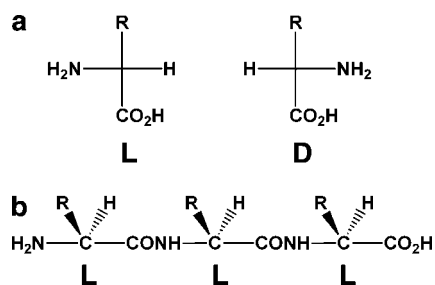
FIGURE 1. (a) The \alpha -amino acids with R \neq H are asymmetric with the possibility of L or D configurational structure. (b) The chains defining proteins are in identical L configuration in every substituted ( R \neq H ) \alpha -carbon.
